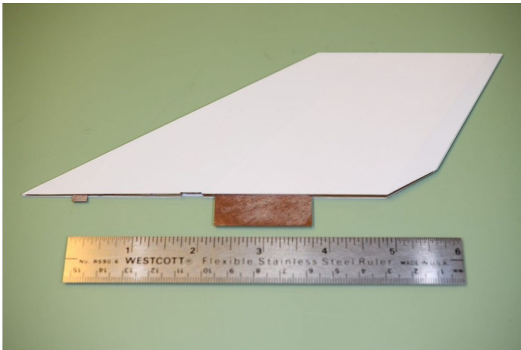
Photo 76: Skinned Fin
