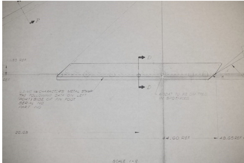
Figure 9: Fin Foot Side View
