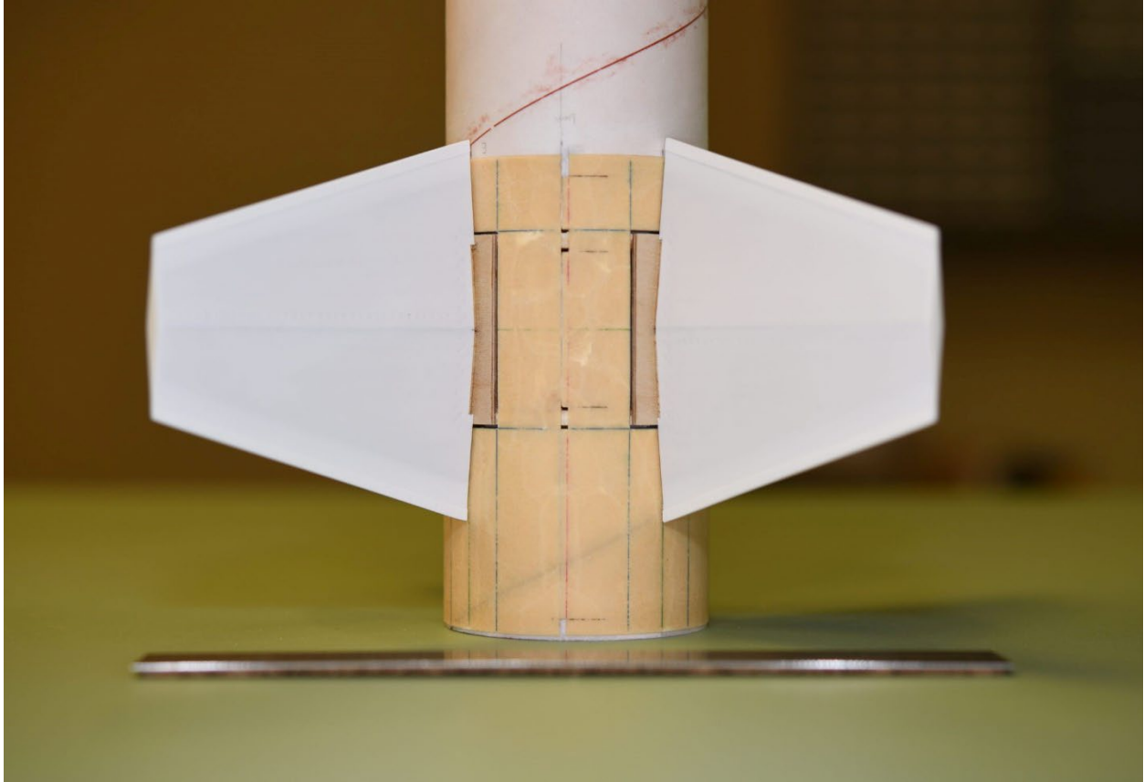
Photo 29: Model Sleeve Seam
