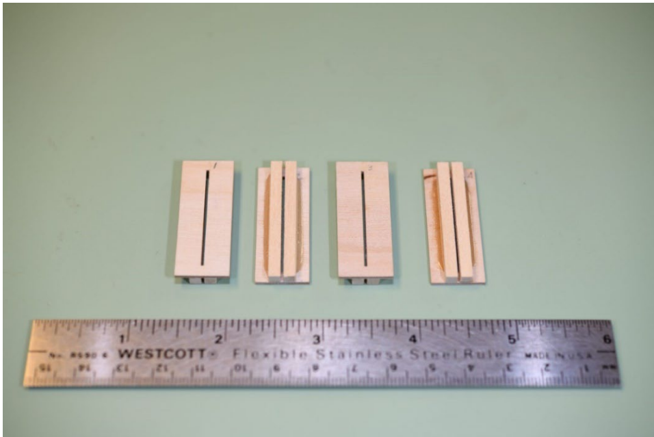
Photo 23: Modified Fin Plates
