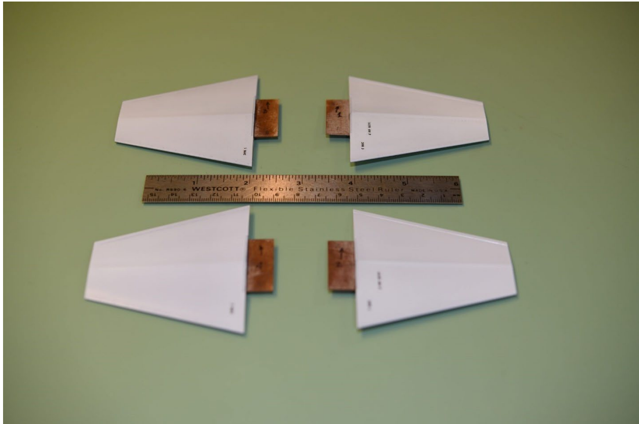
Photo 21: Finished Nike Booster Fins
