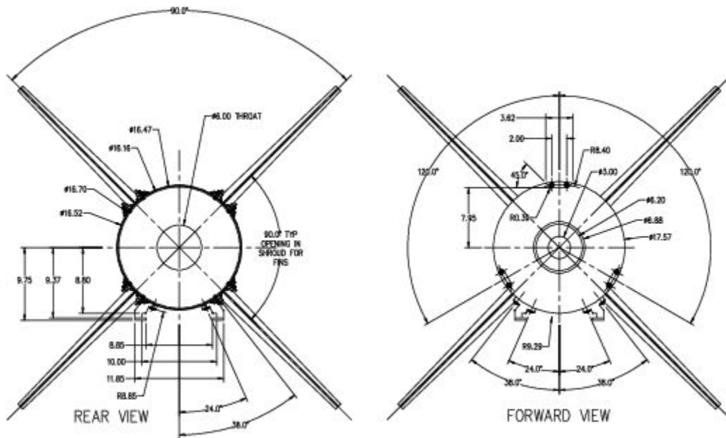
Figure 5: Nike Launch Rail Lugs
