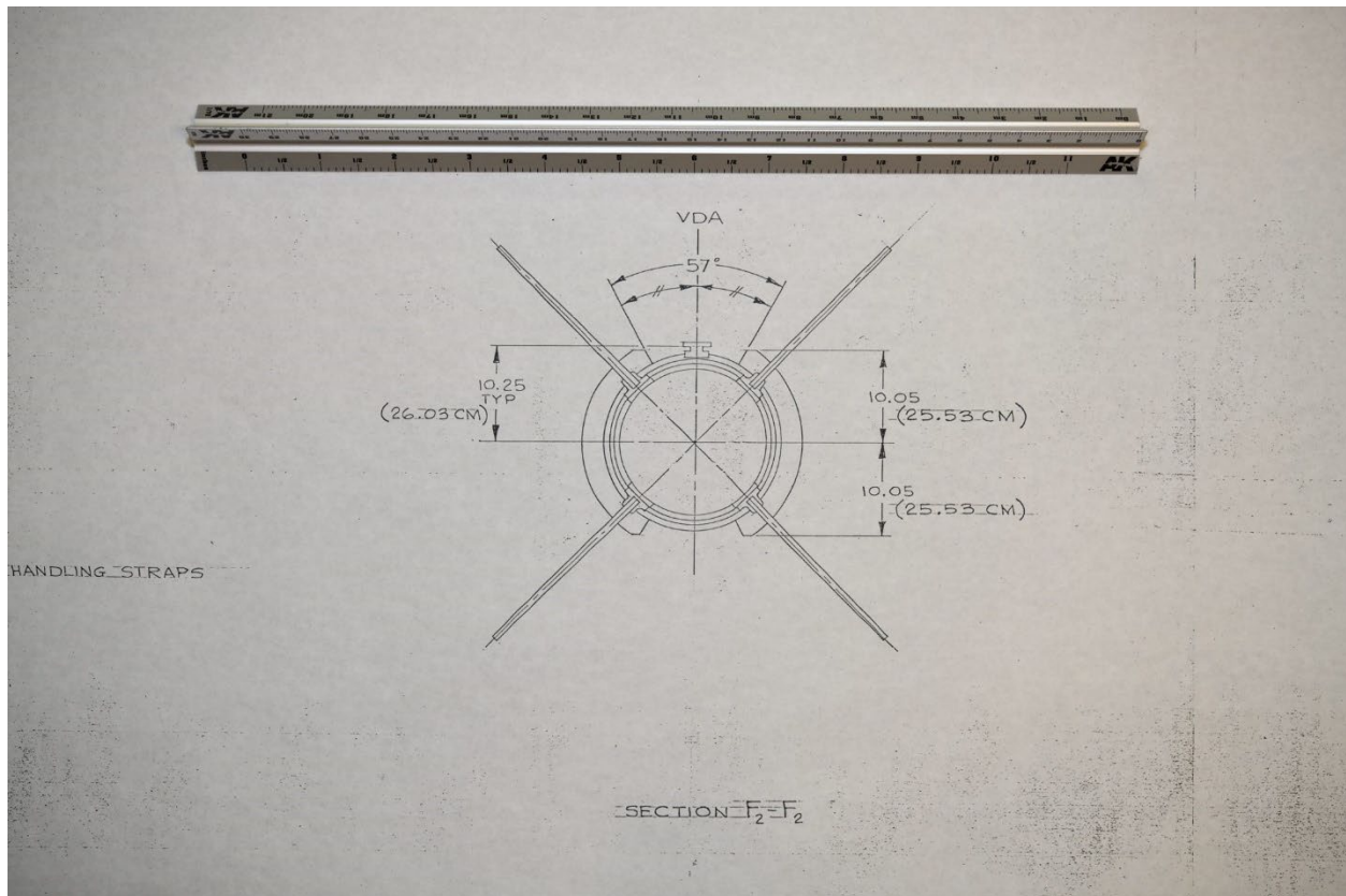
Figure 7: Interstage Adapter Section View
