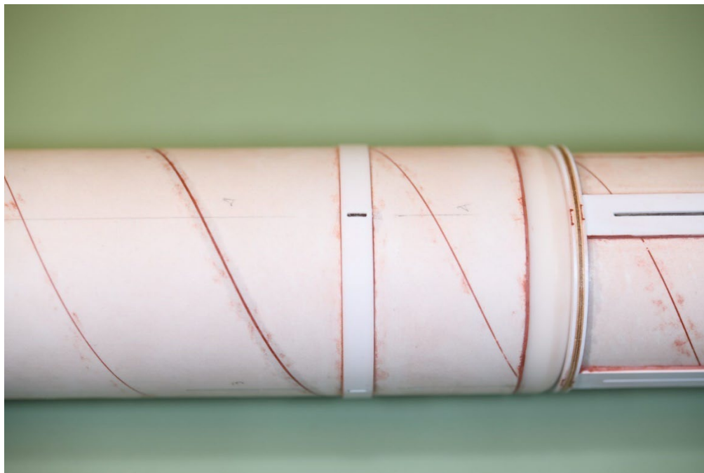
Photo 58: MMT/Fin Can Installed
