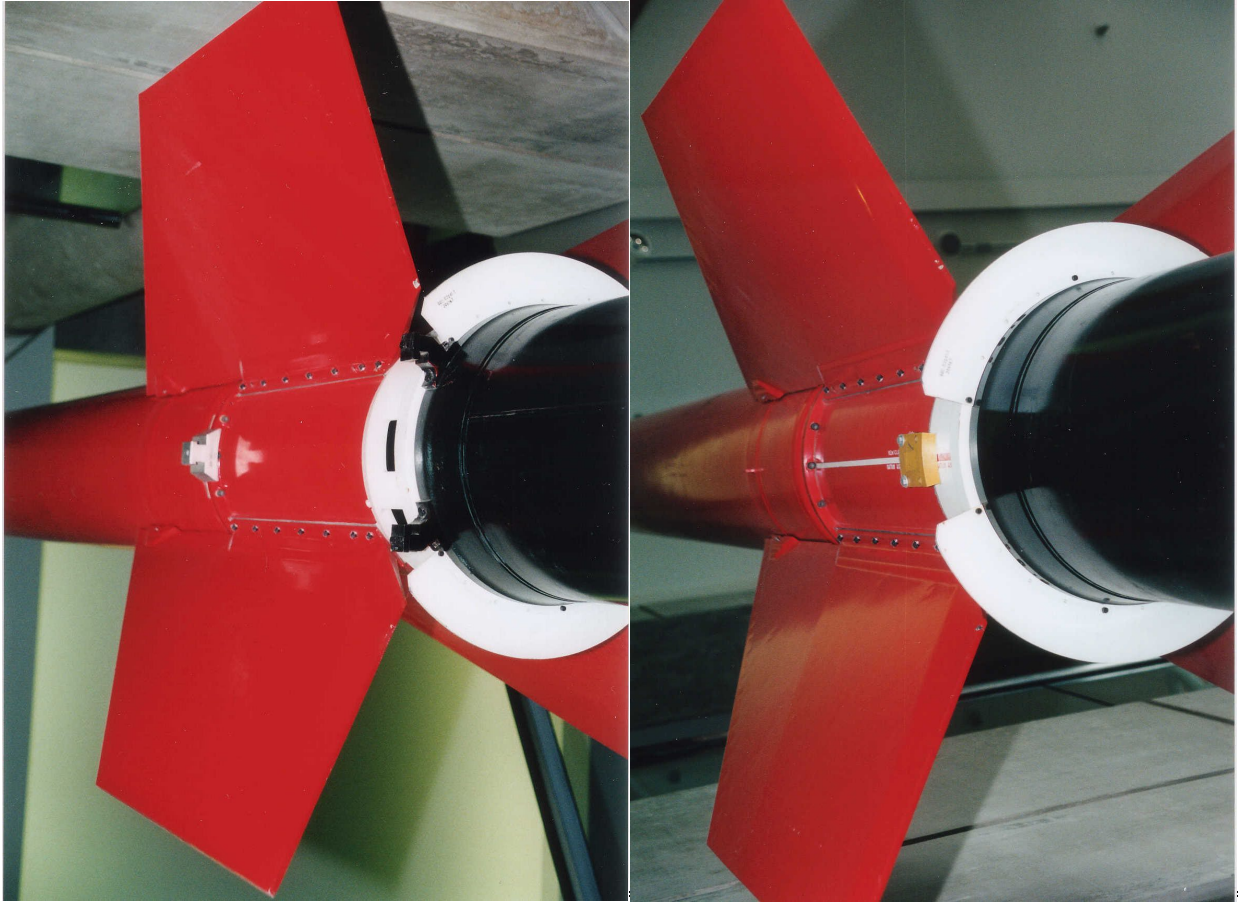
Photo 39: Wide Segment Gap, Left; Narrow Segment Gap, Right
