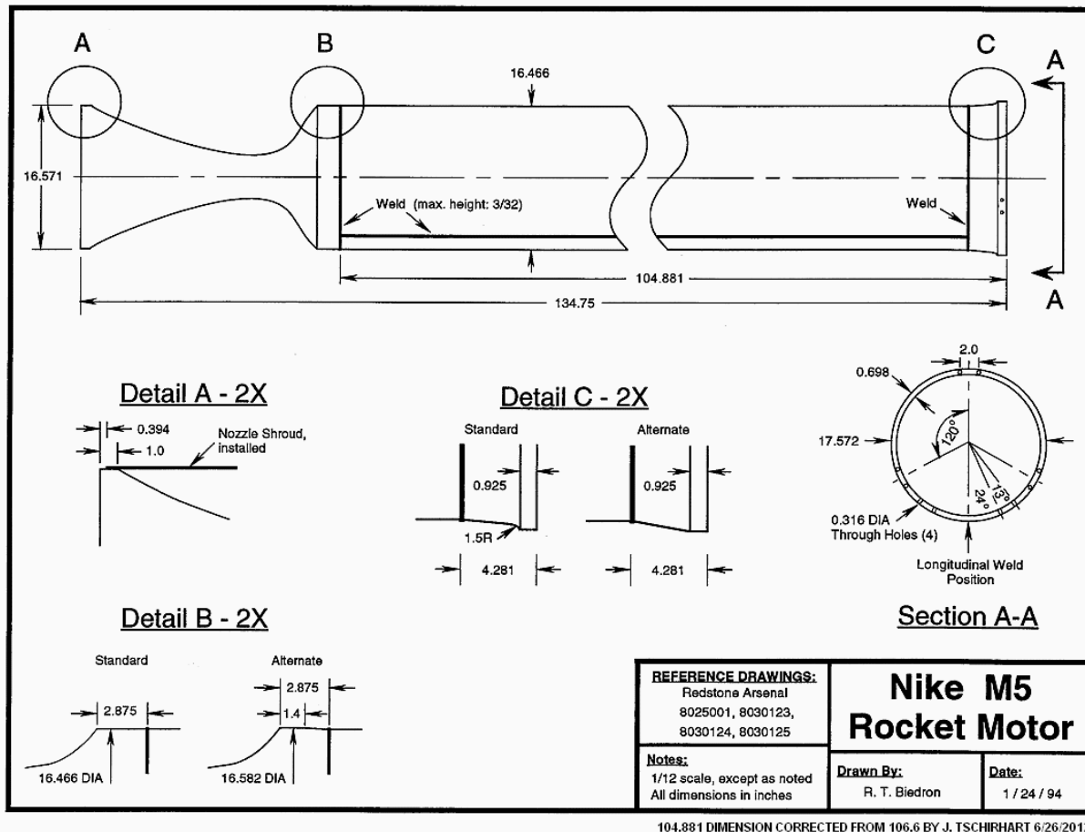
Figure 1: Nike M5 Motor
