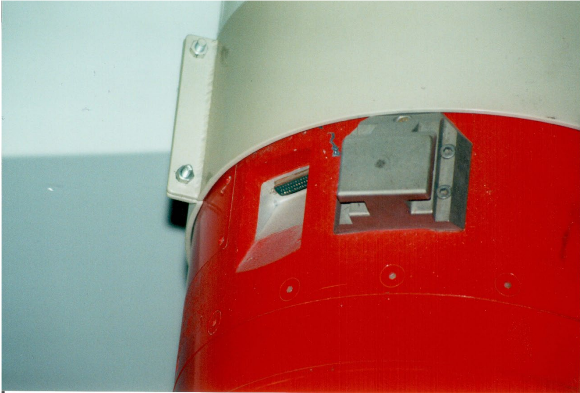
Photo 89: Igniter Housing/Motor Case Joint
