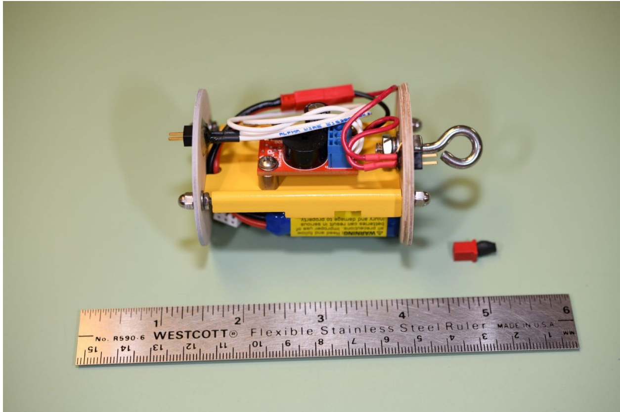
Photo 42: Staging Timer Assembly
