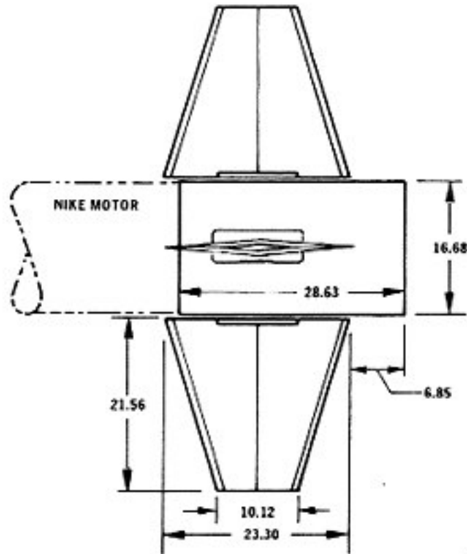
Figure 4: Lightweight Standard Nike Fin
