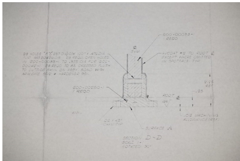
Figure 10: Fin Foot Cross Section
