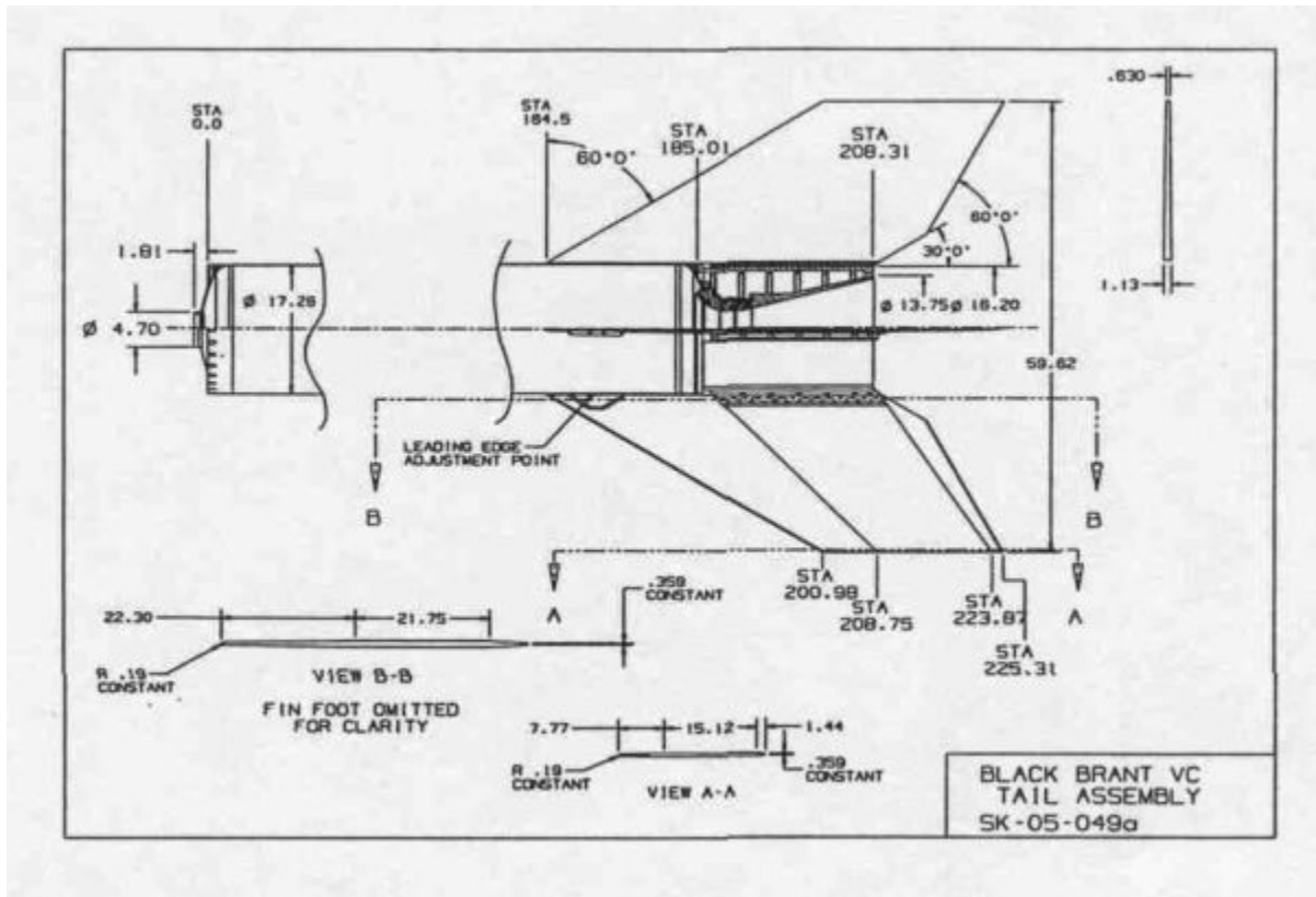
Figure 8: BBVC Tail Assembly
