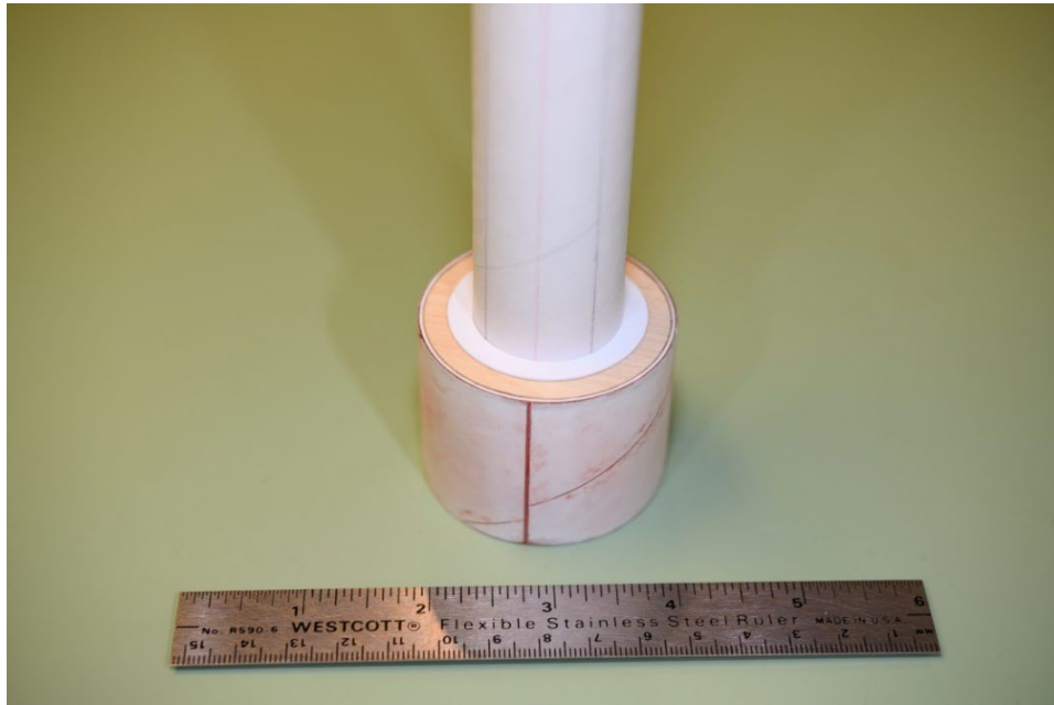
Photo 22: Aft Fin Can
