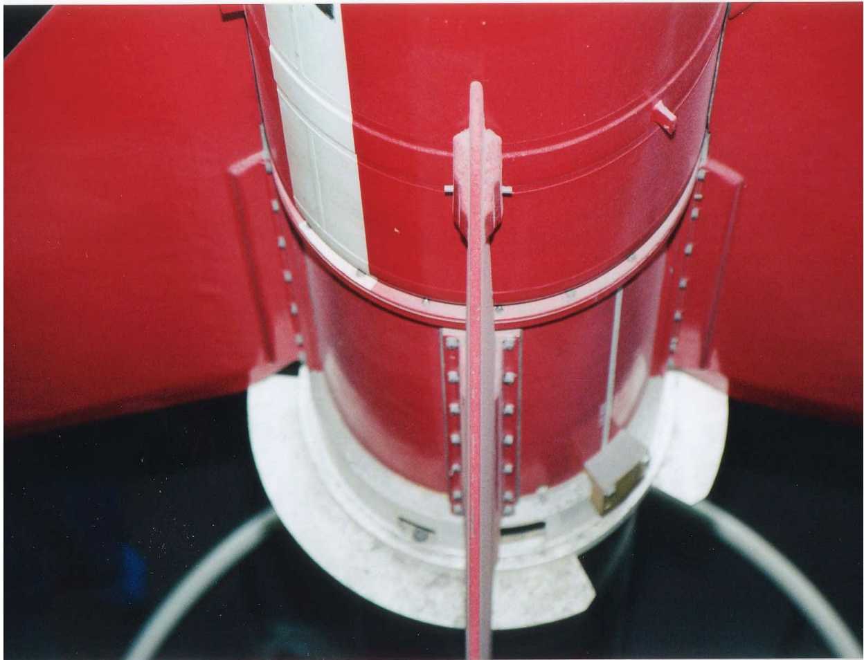
Photo 52: BBVC Motor Case/Fin Can Joint
