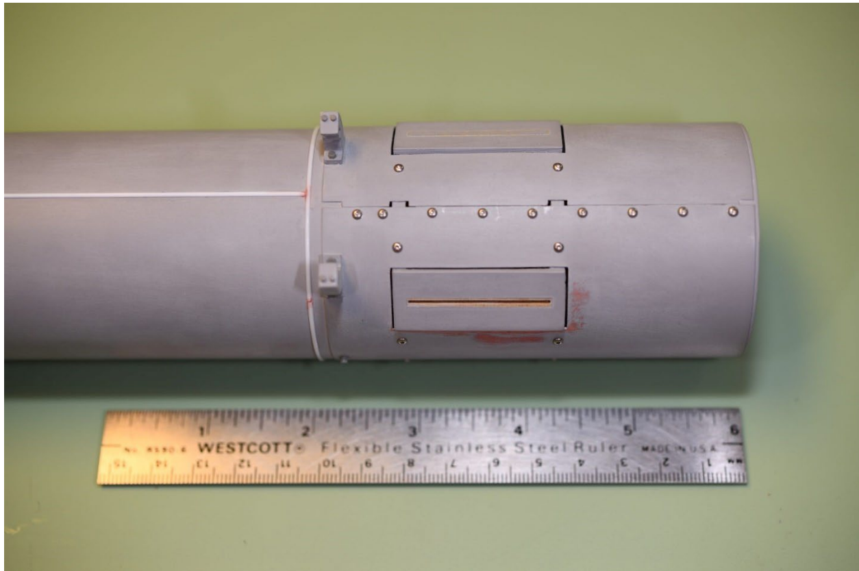
Photo 35: Aft End Details
