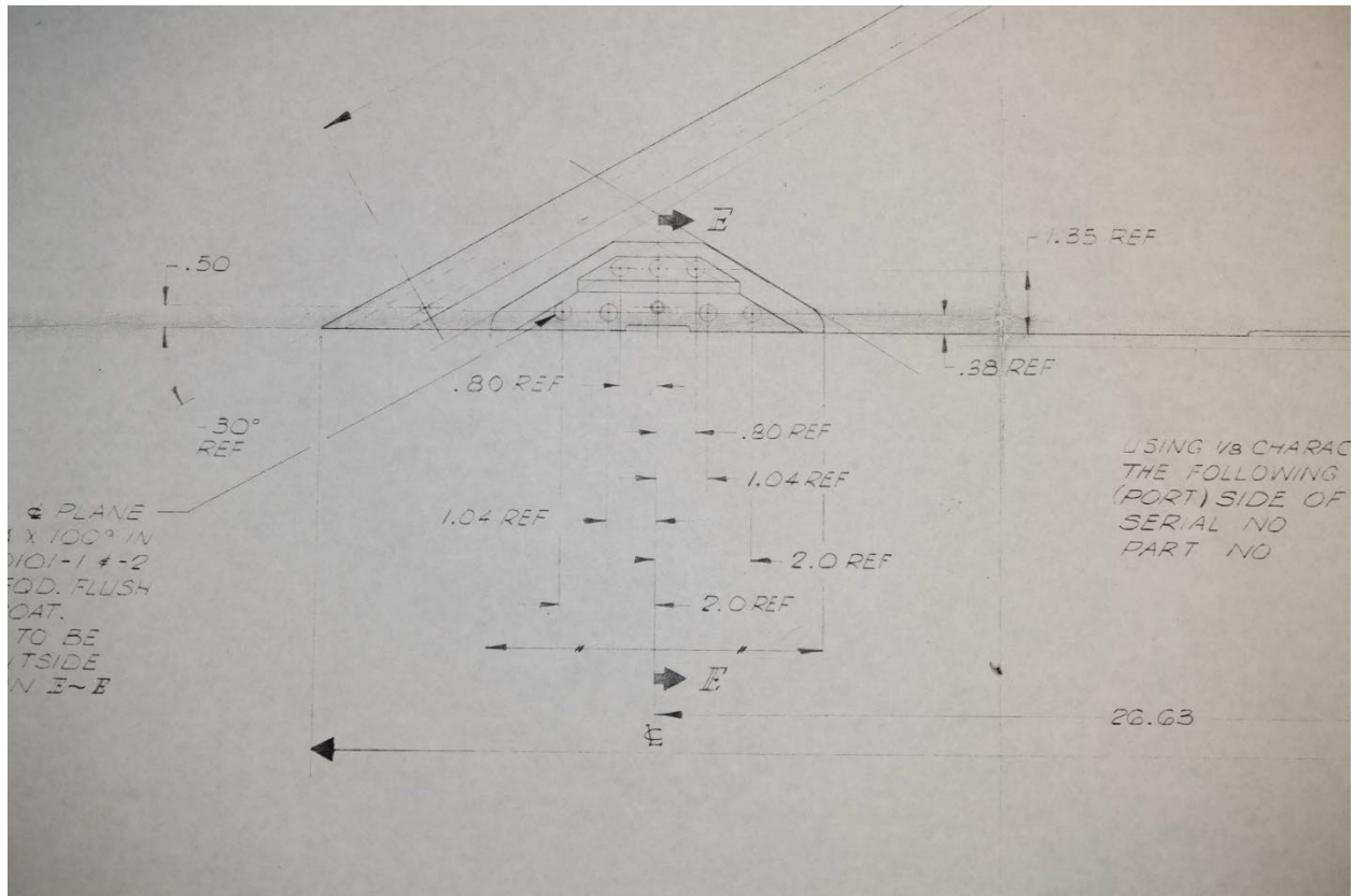
Figure 11: Leading Edge Adjustment Point
