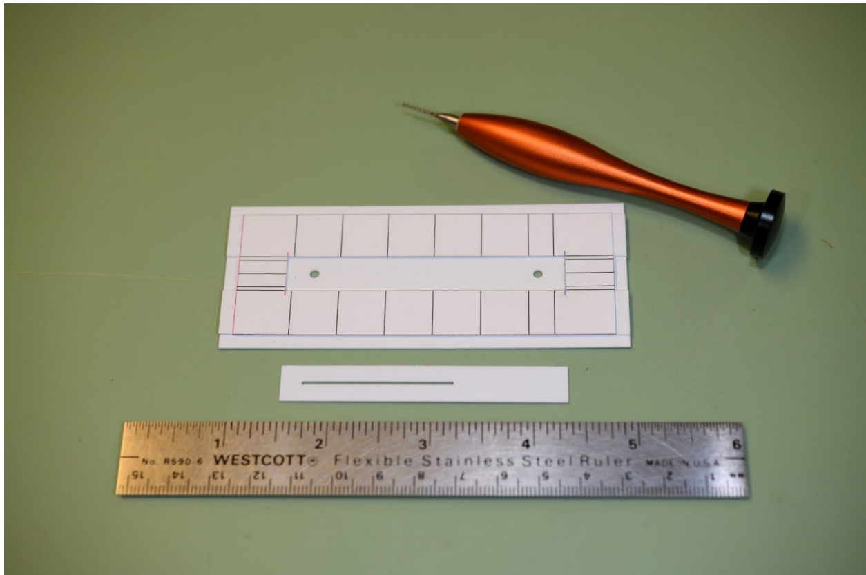
Photo 79: Fin Plate Drilling Jig
