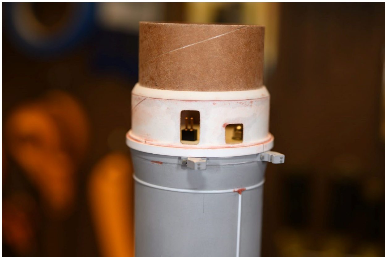
Photo 46: Adapter Trial Fit
