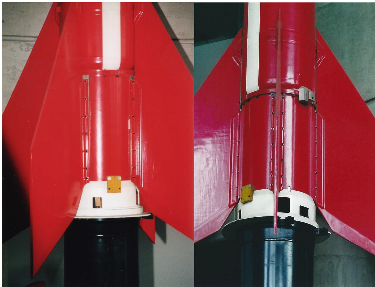
Photo 44: Interstage Adapter
