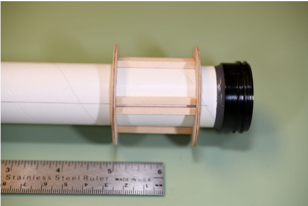
Photo 54: Motor Mount with Fin Tab Wells
