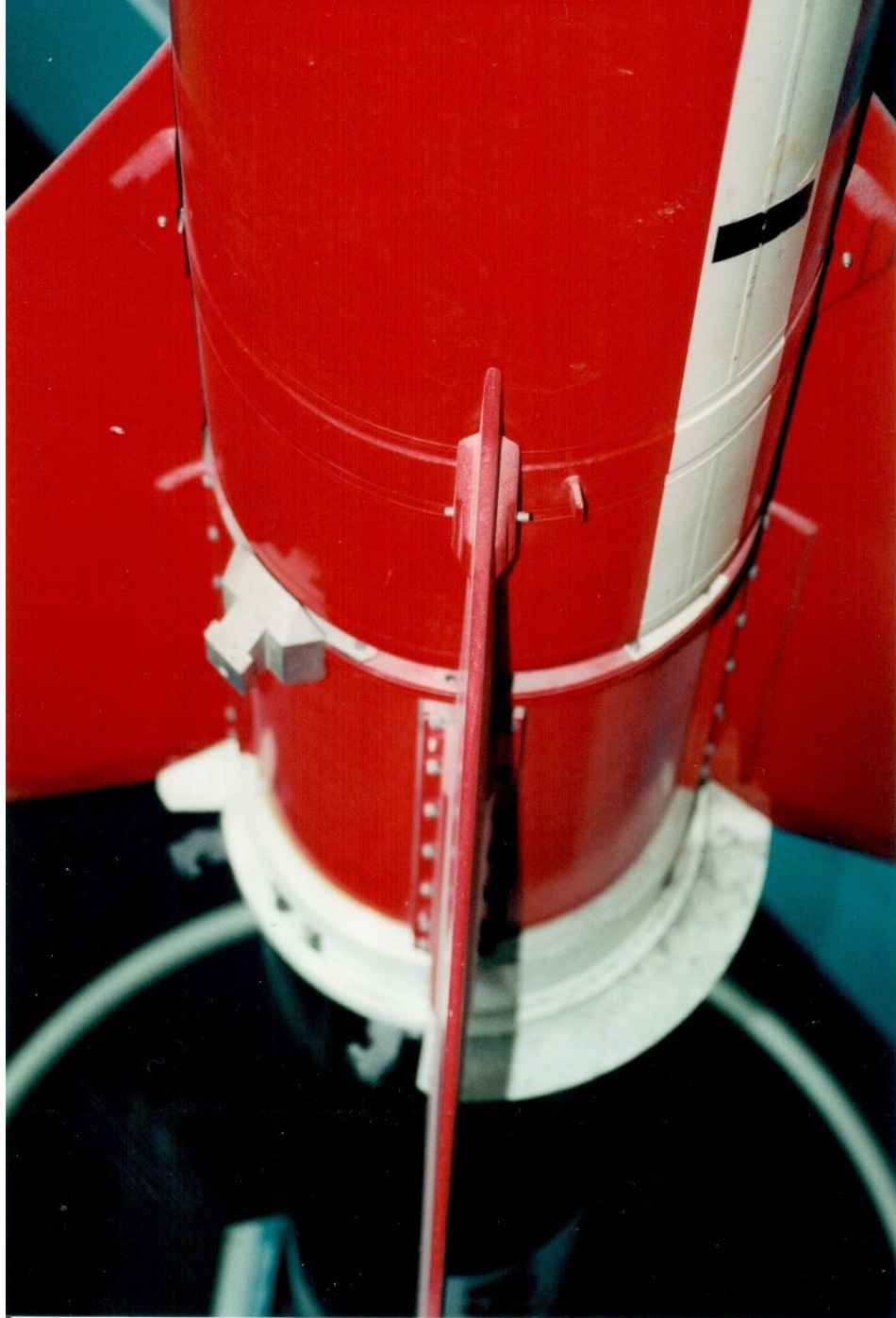
Photo 60: Aft Case Welds
