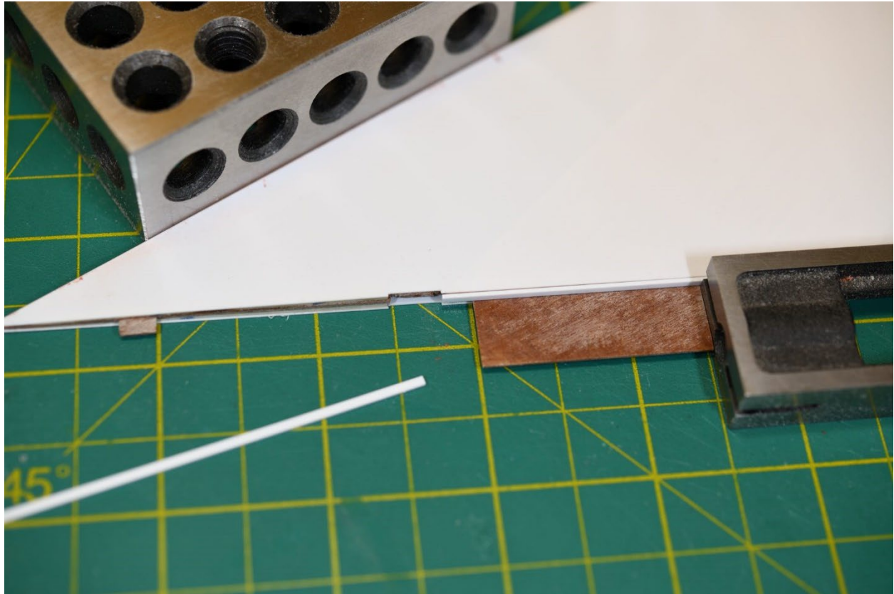
Photo 78: Root Filler Strip
