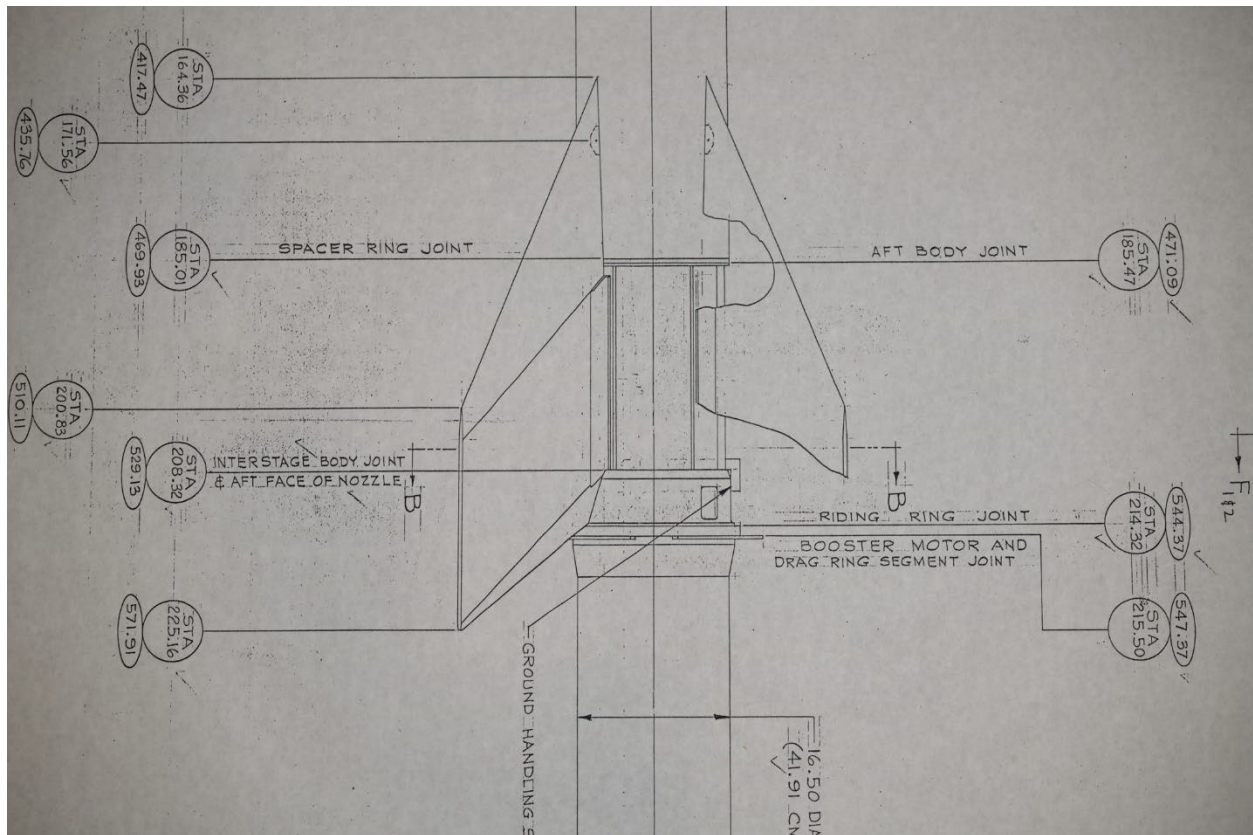
Figure 6: Interstage Adapter Plan View
