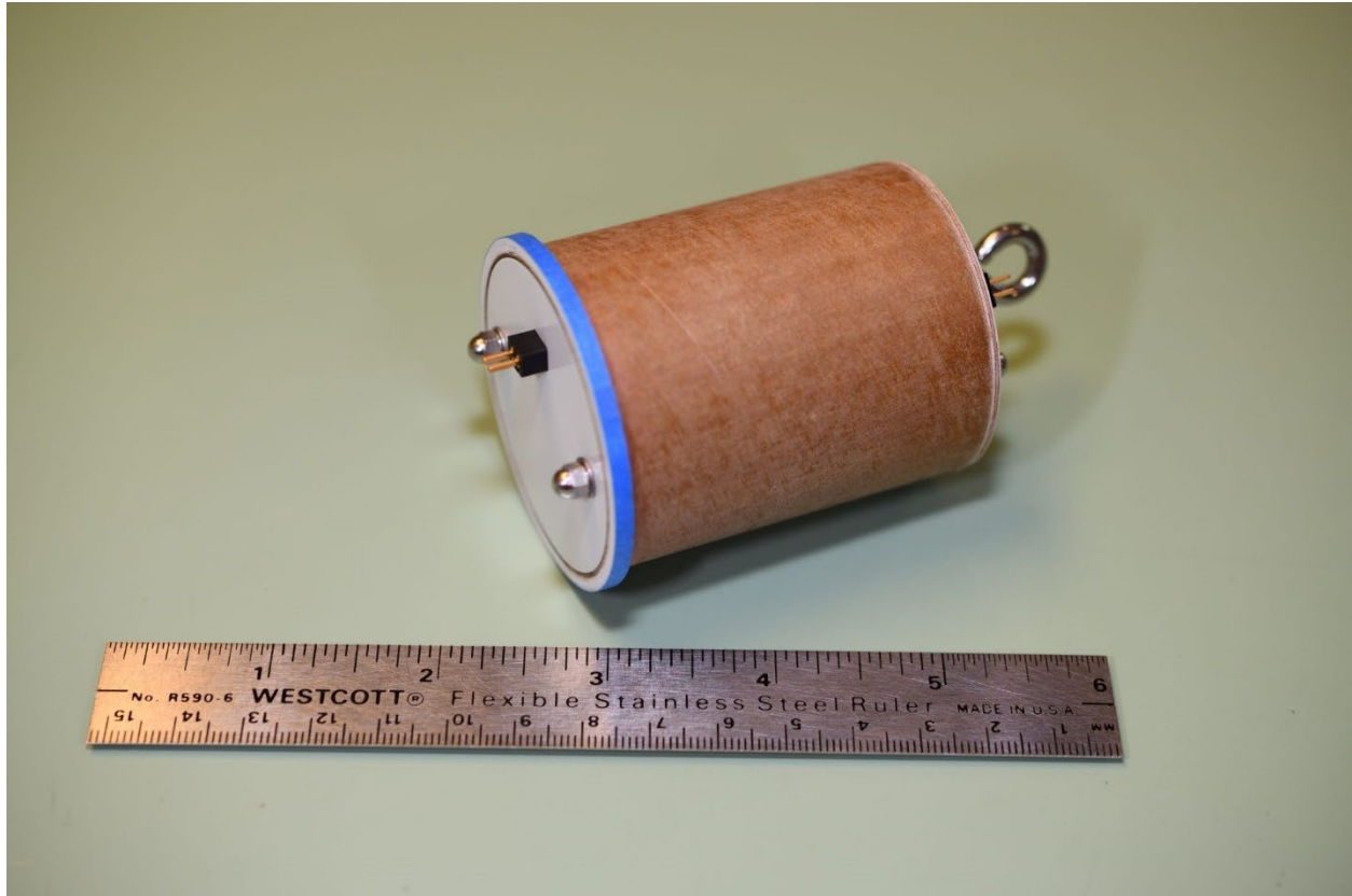
Photo 43: Completed Coupler/Staging Timer Assembly
