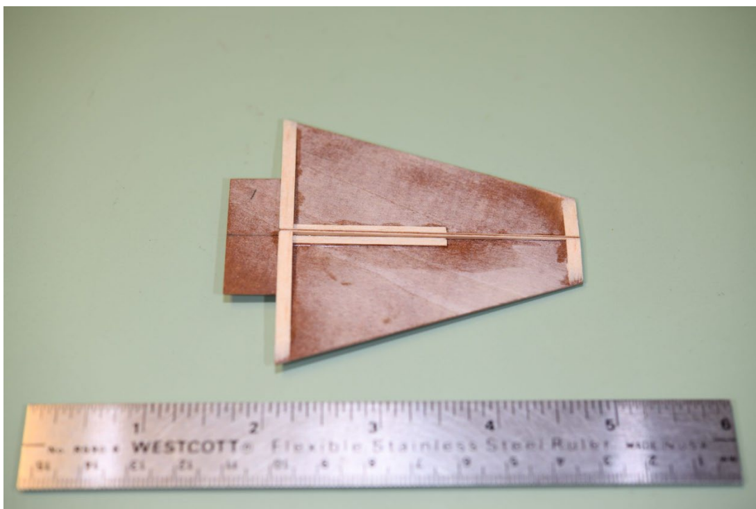
Photo 14: Finished Fin Core
